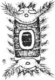
Fig. 90. Saddle back- ed slug caterpillar, Sabine stimulea (Clemens).
